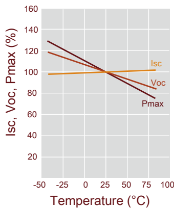
Irradiance: AM 1.5, 1,000W/m 2 (285W)
